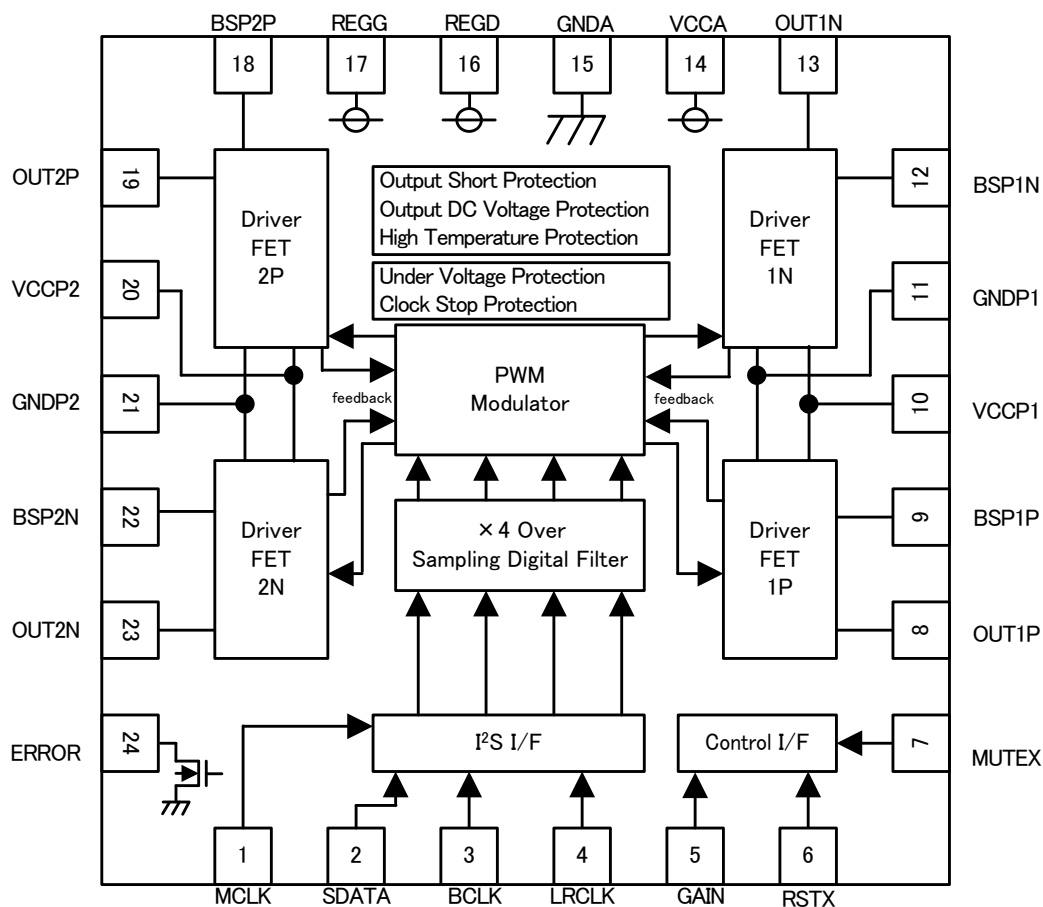
Figure 3. Block Diagram
